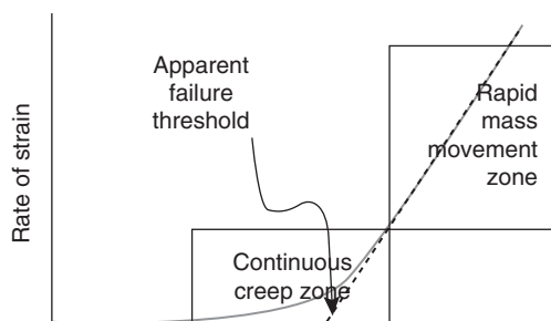
Figure 156 Stress-strain relationship in continuous creep
