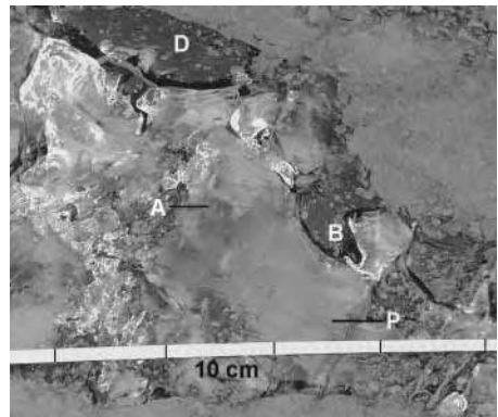
Plate 63 Large crystals of the glacier ice from bottom layers of Horn Glacier, Spitsbergen (intervals of 10 cm are marked). Note inclusions of air bubbles (A), cross section of the crystal basal planes (P), plastically deformed crystal boundaries (B) and presence of debris admixtures (D). Photo by Jacek Jania
