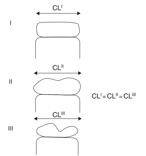
Figure 103 Simple cross-sectional diagrams of three clints demonstrating how plan measures of clint size (CL I , etc.) can be identical on clints with very different degrees of down-wearing
