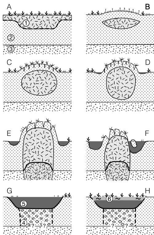
Figure 118 A general model of the formation of the frozen core (1) of a palsa in a mire (2) with a silty till substratum (3). A: the beginning of the thaw season. B: the end of the first thaw season. C: embryo palsa. D: young palsa. E: mature palsa. F: old collapsing palsa surrounded by a large water body. G: fully thawed palsa giving a circular pond on the mire (5). The thawed peat is decomposed (4). H: new peat (6) formation starts in the pond (Seppälä 1982, 1986, 1988)
