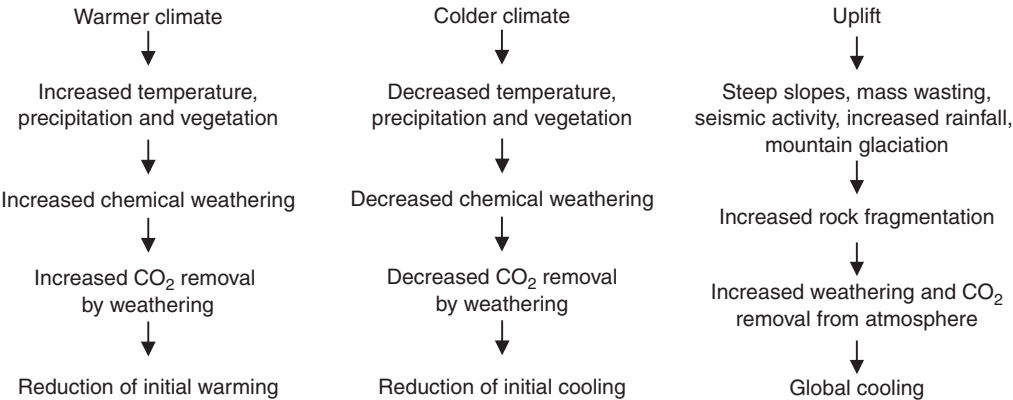
Figure 178 Negative feedbacks between weathering and climate change
