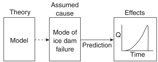
Figure 114 Schematic representation of the deductive mode of palaehydrological inference applied to the problem of predicting an outburst flood hydrograph from a general theory for the failure of an ice-dammed lake
