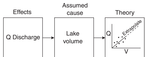
Figure 115 Schematic representation of the inductive mode of palaehydrological inference applied to the problem of estimating the relationship between lake volume and peak outflow discharge for the failure of ice-dammed glacial lakes
