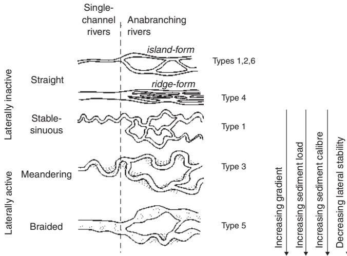
Figure 5 A classification of river channel patterns including single channel and anabranching plan-forms. Laterally inactive channels consist of straight and sinuous forms whereas laterally active channels consist of meandering and braided forms. The anabranching types are described in the text (after Nanson and Knighton 1996)
