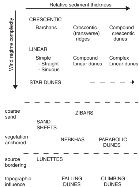
Figure 50 The main dune morphological types
