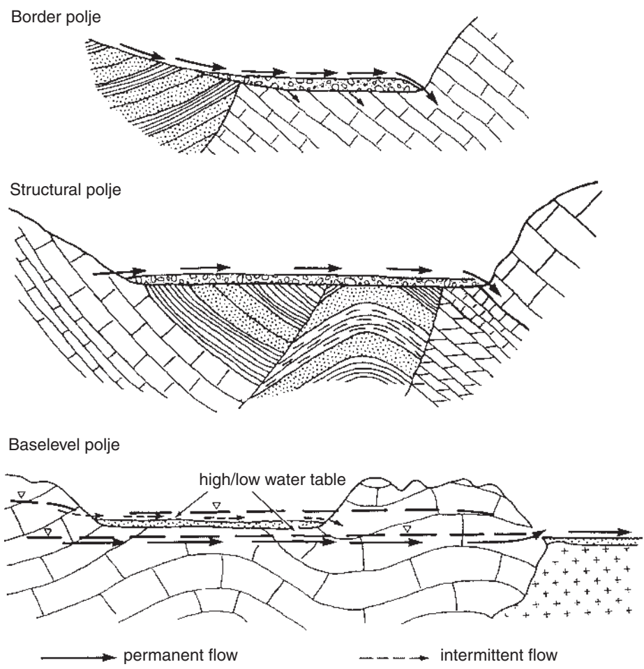
Figure 98 Three main types of polje. These are the largest enclosed depressions found in karst landscapes. Their flat floors are prone to flood and may cover many square kilometres in area (from Ford and Williams 1989.)
