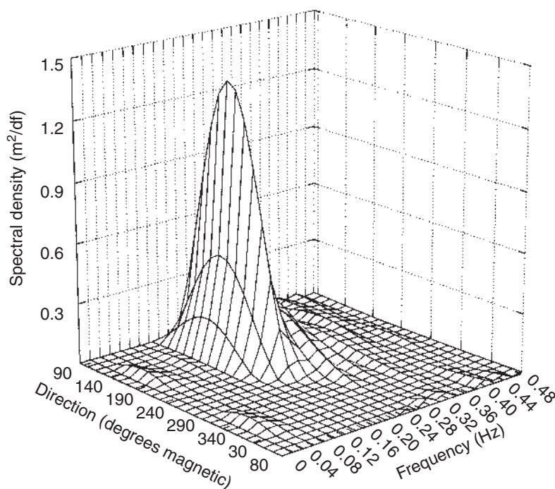
Figure 175 Directional wave spectrum recorded from southern Lake Huron, Canada in ~8 m water depth ~2 km offshore, recorded using a Falmouth Scientific 3DACM Wave Recorder. The record represents a 20-min sample of water surface elevation collected at 2 Hz. Note: a standard frequency spectrum can be obtained by simply projecting the data onto the left-hand frame. These waves have a peak period of ~5 s and a peak direction of approach between 160° and 170°
