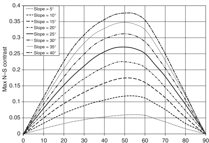
Figure 8 Difference in total annual radiation between north and south-facing slopes for clear sky conditions
