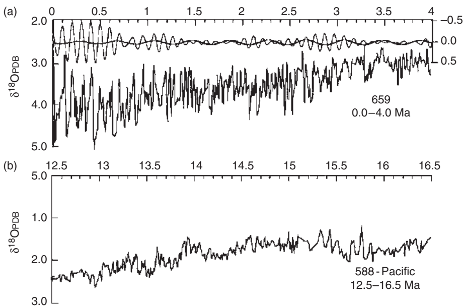
Figure 146 Contrasting records of marine oxygen isotopes from 0–4 Myr (Plio-Pleistocene) and 12.5–16.5 Myr (Miocene). The increase of amplitude in \delta^{18}\text{O} cycles around 2.6 Myr represents the onset of large fluctuations of ice sheets and sea level, which become even more pronounced around 1 Myr, when they adopt a characteristic period of \sim 100,000 years. The upper curve in (a) shows the changing amplitude of the 100,000 year cycle (after Zachos et al. 2001)
