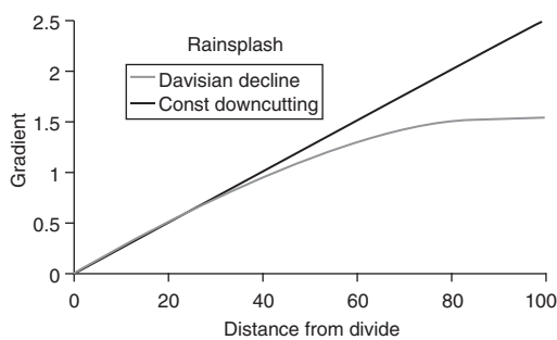
Figure 152 Slope evolution where rainsplash is dominant
