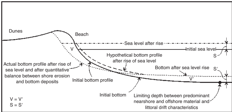
Figure 15 The Bruun Rule implies that the sediment volume removed from the beach and nearshore ( V ) must equal the sediment volume on the lower shoreface ( V' ) and that the lower shoreface aggrades in direct proportion ( S' ) to the rise in sea level ( S ). (After Bruun 1962 and Dubois 2002)
