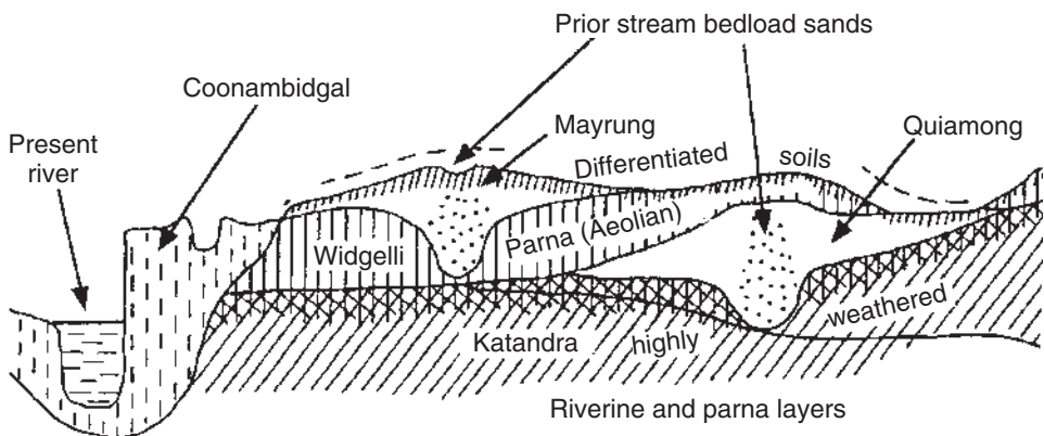
Figure 128 Generalized cross section of Riverine Plain showing Butler's (1958) prior stream sediments and soils (grounds) surfaces
