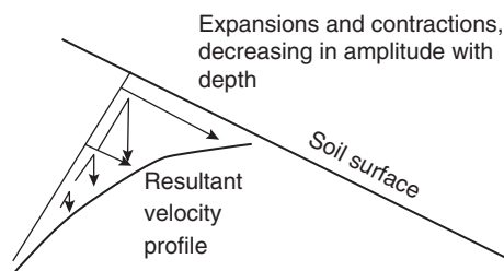
Figure 157 Zigzag seasonal creep movement
