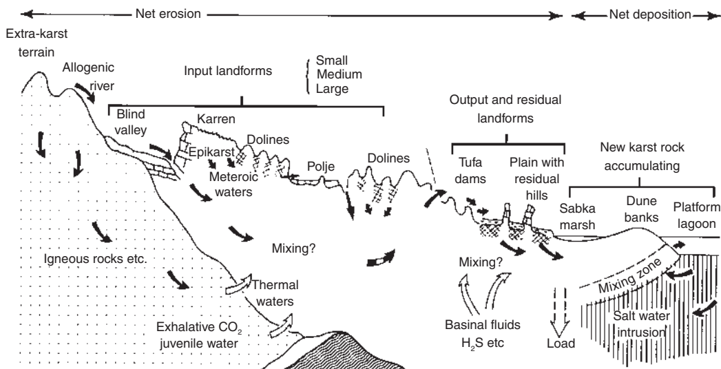
Figure 96 A conceptual model of the comprehensive karst system (from Ford and Williams 1989.)
