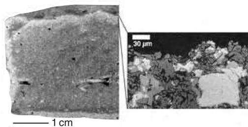
Plate 96 Weathering rind developed on a glacially polished basalt, Mauna Kea, Hawaii. This rind developed over a 16,000-year period. The left photograph shows an optical rind visible in a hand specimen. The right image shows an electron microscope (backscatter) image of a small section of the rind, illustrating three aspects of rind development. First, dissolution of minerals dominates rind formation, as exemplified by the pores (black areas). Second, the bright spots in the image are reprecipitated iron hydroxides, responsible for reddening. Third, rinds may not necessarily thicken over time. Often, they undergo erosion as pieces of weathered minerals progressively detach, that is if rinds are not protected by rock coatings
