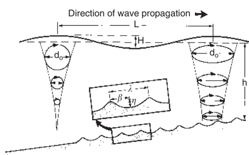
Figure 174 Schematic of wave form and water particle motion in deep and shallow water, where the wave form interacts with a rippled bed. Note: L = wave length; H = wave height; d_0 = orbital diameter; h = water depth
