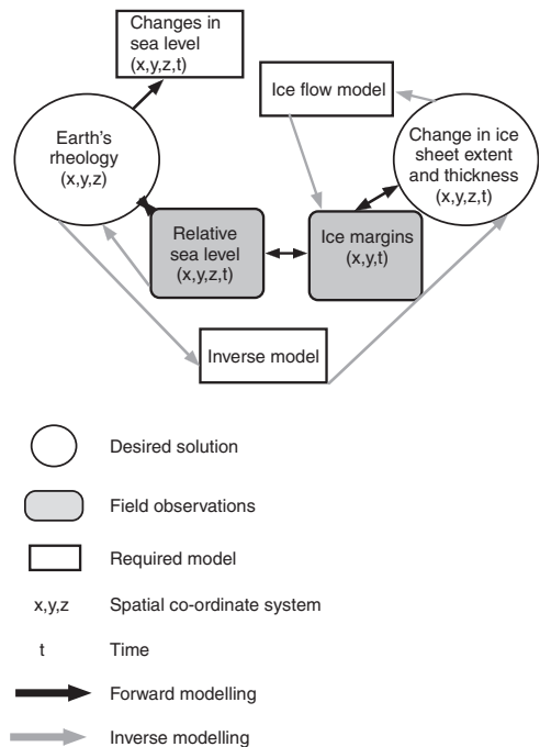
Figure 70 Schematic diagram on interactions between data and models
