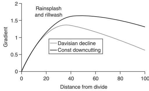
Figure 153 Slope evolution with rainsplash and rillwash
